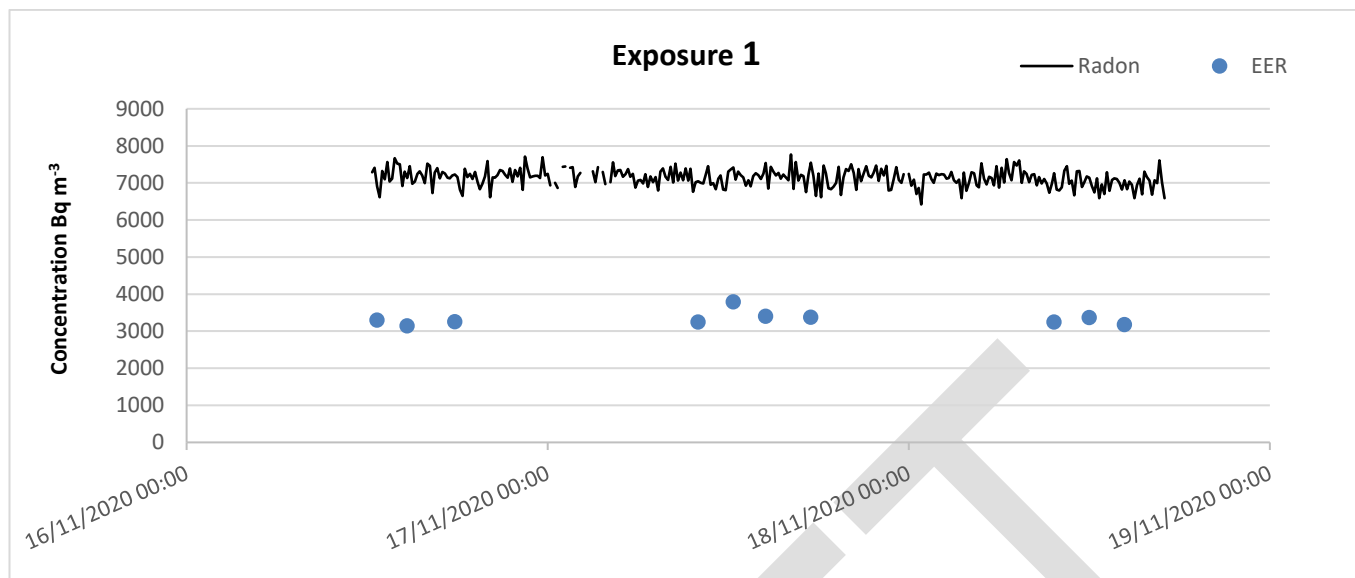
Figure 1. Radon and EER concentrations for exposure 1
