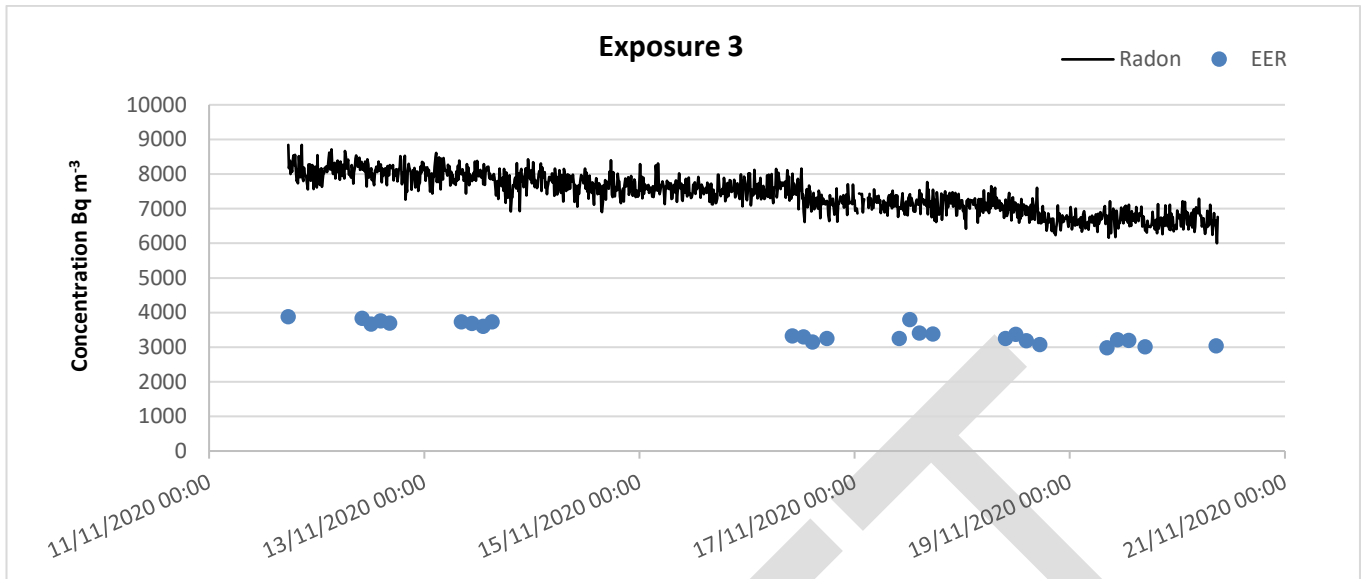
Figure 3. Radon and EER concentrations for exposure 3
